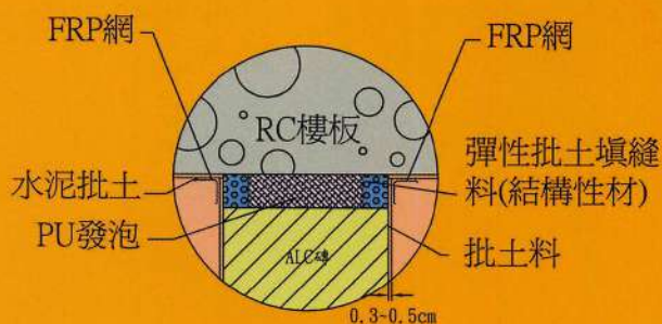
(C) RC樑、樓板與ALC磚
