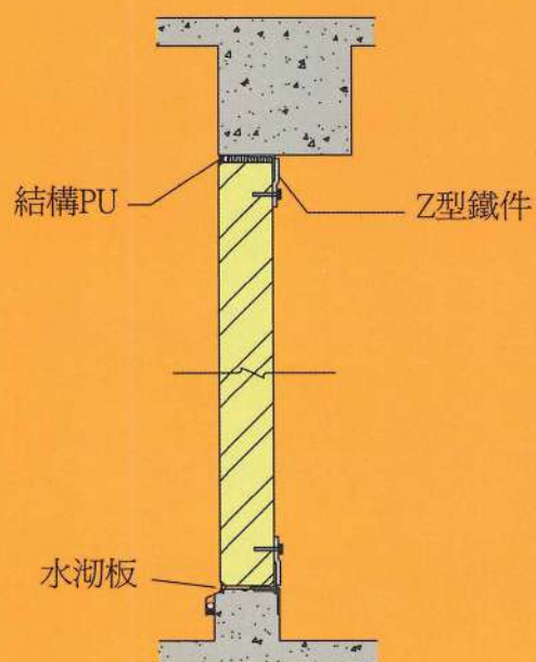
①h3 退縮陽台牆
